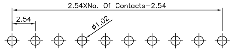
△ Recommended P.C.B. Layout(Top View) (PCB Board Tolerance±0.05)
