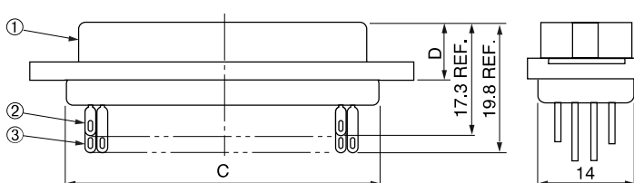
60-contact connector
