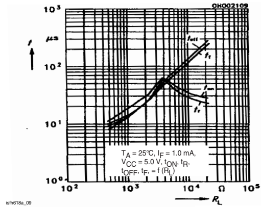
Fig. 11 Switching times (typ.)
