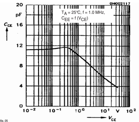
Fig. 8 Transistor Capacitance
