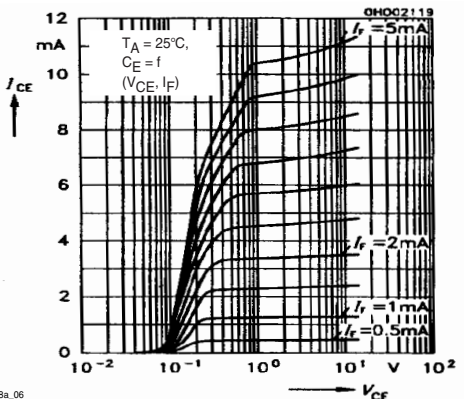
Fig. 9 Output Characteristics
