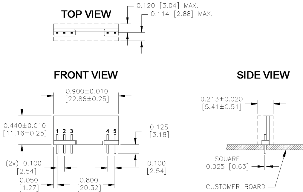
YNV05T06 Pinout (Through-Hole - SIP)
