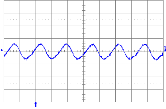
Fig. 3.3V.6: Output voltage ripple (20mV/div.) at full rated load current into a resistive load with external capacitance 47\mu F ceramic + 1\mu F ceramic and V_{in} = 5V for V_{out} = 3.3V . Time scale: 2\mu s /div.
