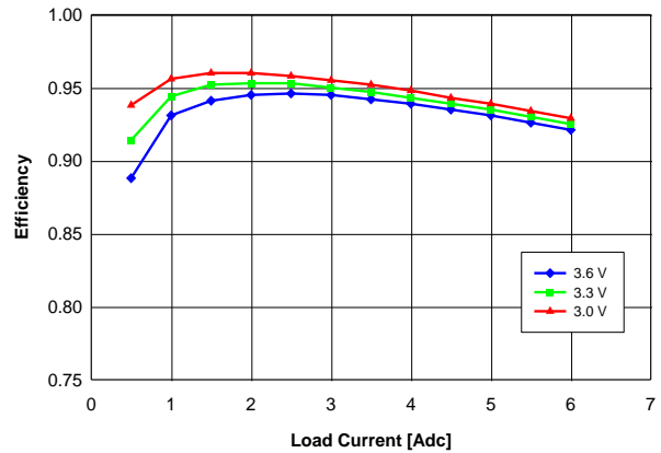
Fig. 2.5V.4: Efficiency vs. load current and input voltage for V_{out} = 2.5V converter mounted vertically or horizontally with air flowing from pin 5 to pin 1 at a rate of 200 LFM (1 m/s) and T_a = 25^{\circ}C .
